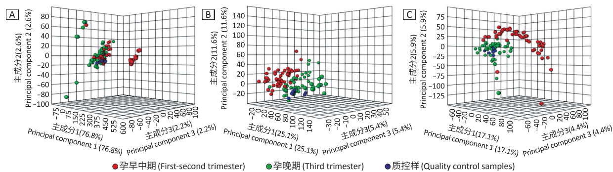
[注] A：UHPLC-QE-MS 阳离子模式；B：UHPLC-QE-MS 阴离子模式；C：GC-TOF-MS。 [Note] A: UHPLC-QE-MS positive ion mode; B: UHPLC-QE-MS negative ion mode; C: GC-TOF-MS. 图1 质控样本GC-TOF-MS及UHPLC-QE-MS主成分分析结果 Figure 1 Principal component analysis results of quality control samples by GC-TOF-MS and UHPLC-QE-MS
